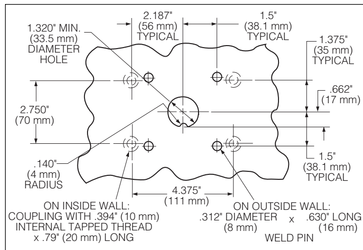
Figure 6a. Hole, coupling and weld pin placement (Bolt-in system).
