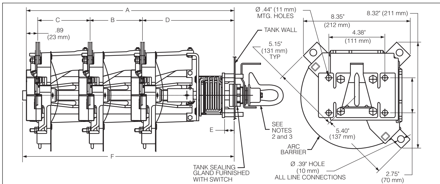
Figure 5. Line illustration with dimensions of sectionalizing switch with “Bolt-In System.”
