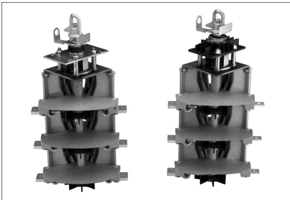
Figure 1. Sectionalizing Switches. Three-phase Bolt-In (left) and three-phase Quick-Mount (right).
