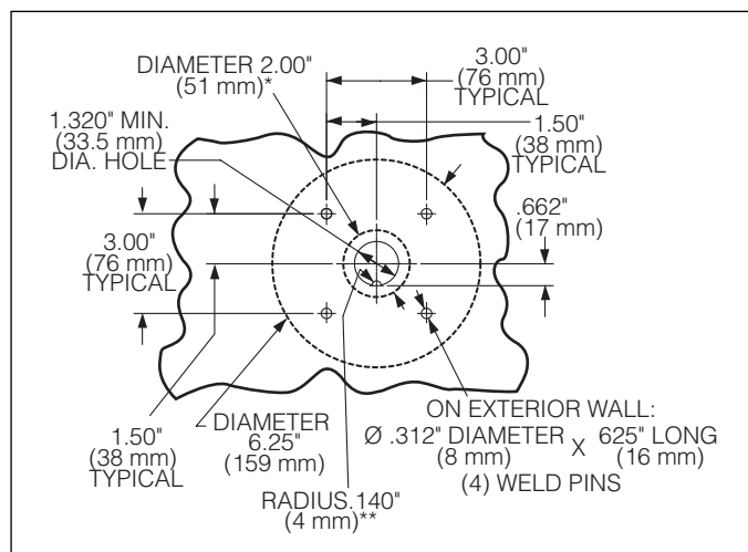
Figure 6b. Hole and weld pin placement (Quick-Mount system).
